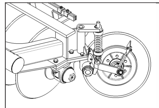
Coulter Disc Assy.
